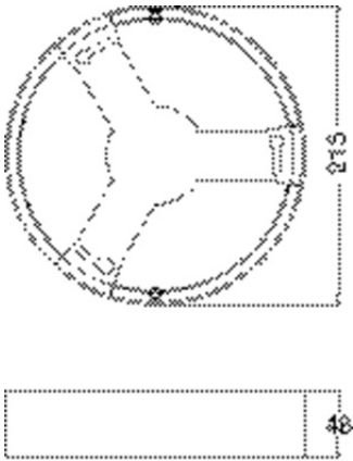
DL IP44 FRAME DN 215
