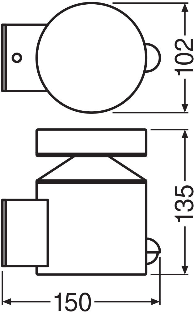
Product line drawing with numbers
