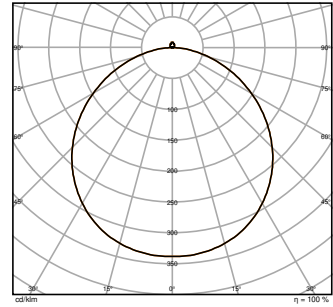
SF C 500 19W WHITE FRAME 1400lm
